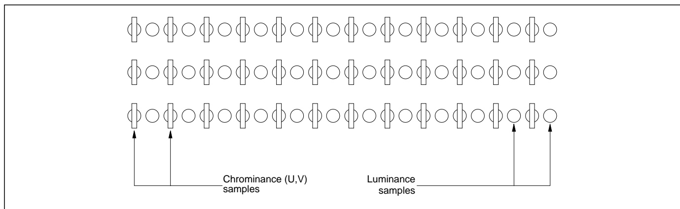
Figure 6-5. Camera YUV 4:2:2 sampling (co-sited luminance/chrominance).
