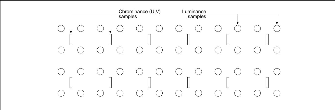
Figure 7-21. YUV 4:2:0 format.
