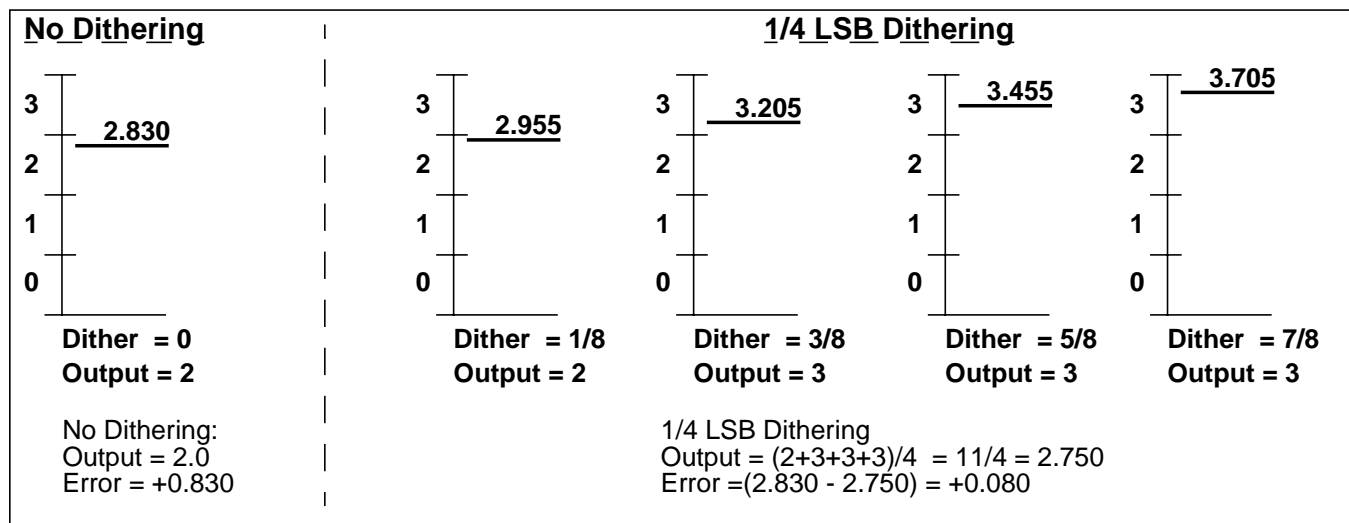
Figure 14-10. Dithering
